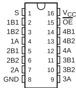
DGX OR PW PACKAGE (TOP VIEW)
