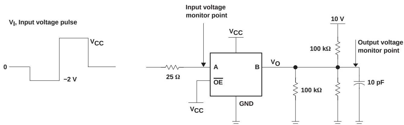
Figure A-6. SPICE Simulation Setup for Undershoot Measurement
