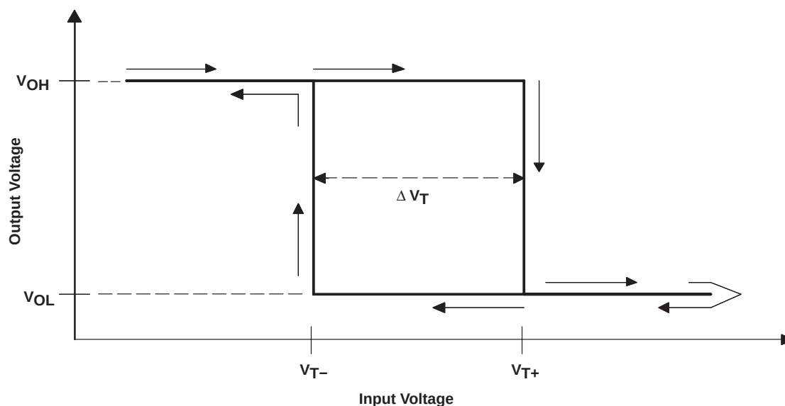
Figure 22. Hysteresis: V_I vs V_O
