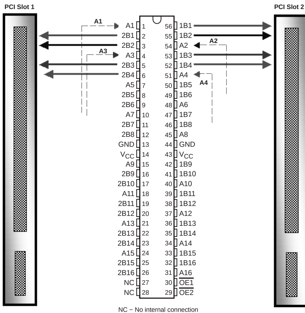
Figure 15. Example of Bus Isolation Using a CBT-C Device
