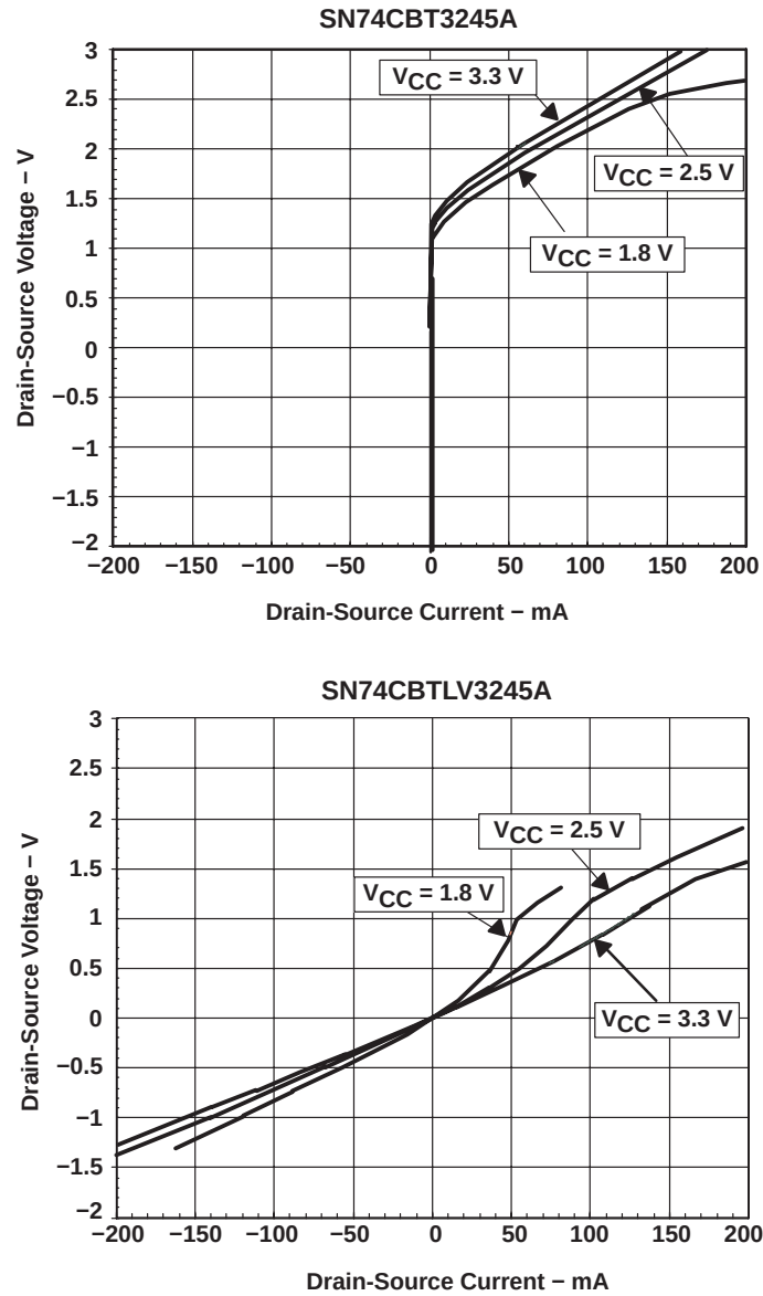
Figure 9. High-State r_{on} of CBT3245A and CBTLV3245A at Different Supply Voltages
