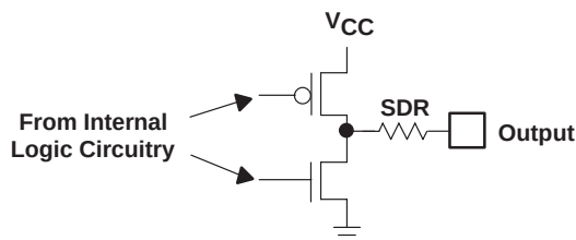
Figure 15. Series-Damping-Resistor Option
