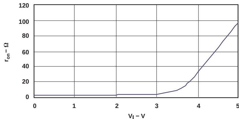
Figure 4. r_{on} vs V_I Characteristic of an NMOS Series Switch ( V_{CC} = 5 V, I_O = -15 mA)
