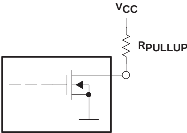
Figure 16. Open-Drain Output Principle
