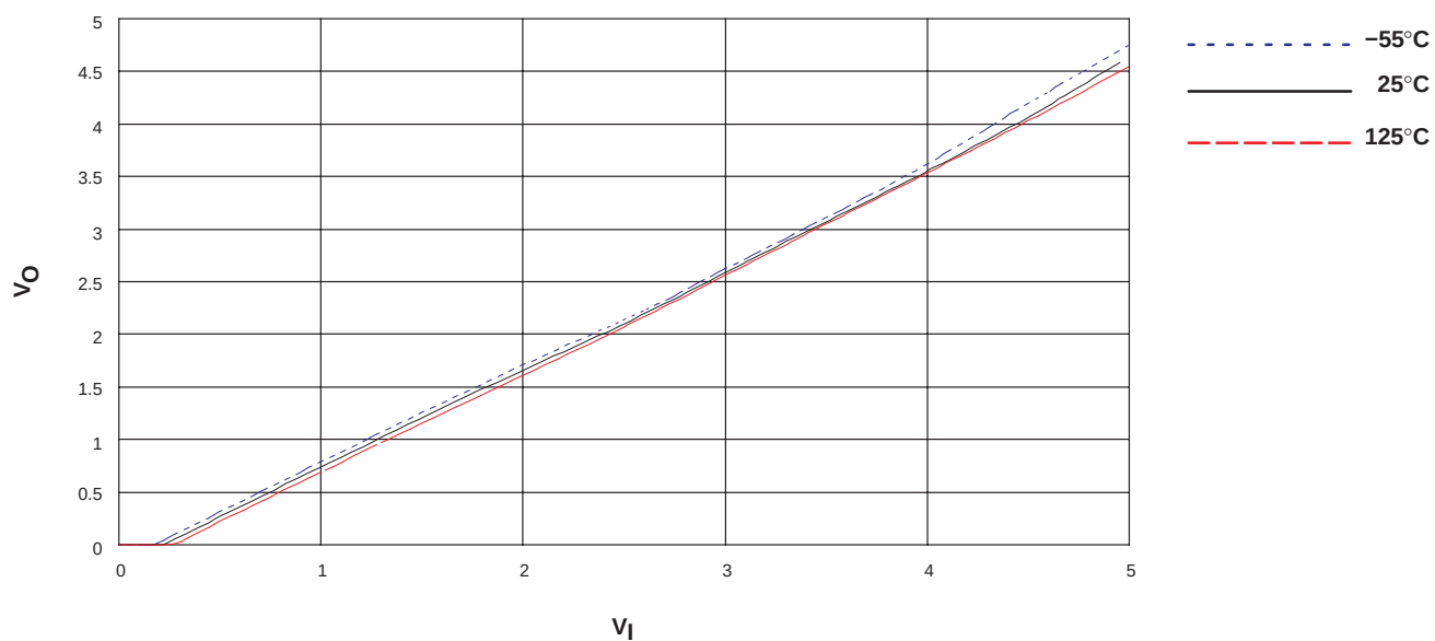
Figure 24. V_O vs V_I , V_{CC} = 5\text{ V} (CD4066B)
