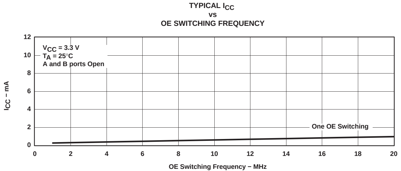
Figure 2. Typical I_{CC} vs OE Switching Frequency, V_{CC} = 3.3\text{ V}
