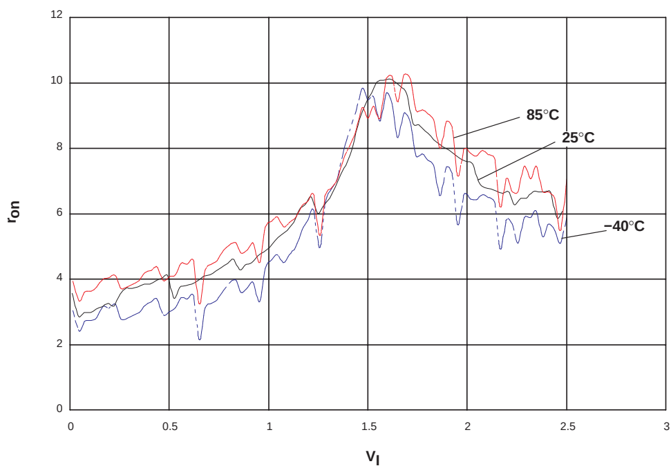
Figure 47. r_{on} vs V_I , V_{CC} = 2.5 V (SN74CBTLV3125)
