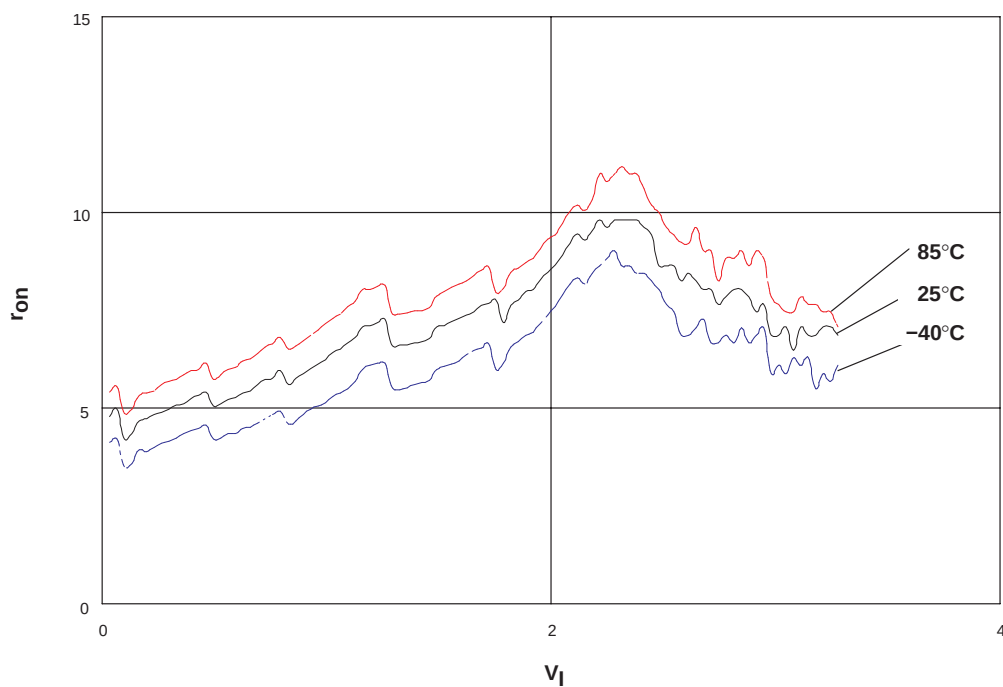
Figure 43. r_{on} vs V_I , V_{CC} = 3.3 V (SN74LVC1G66)
