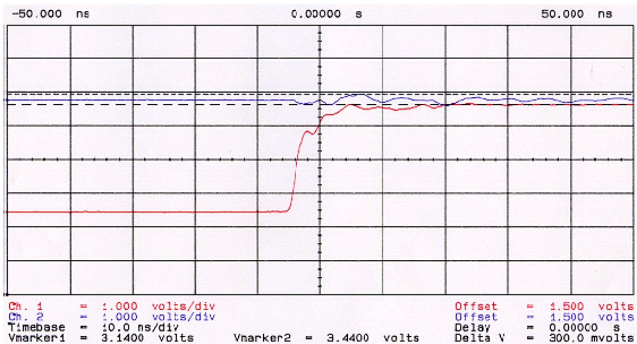
Figure 10. Simultaneous-Switching Plot for CBTLV16292 ( V_{OHV} , V_{OHP} )
