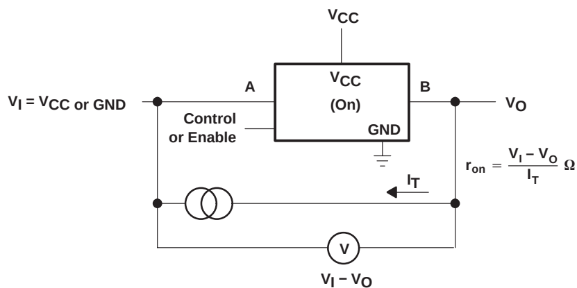
Figure A-1. r_{on} Test Circuit
