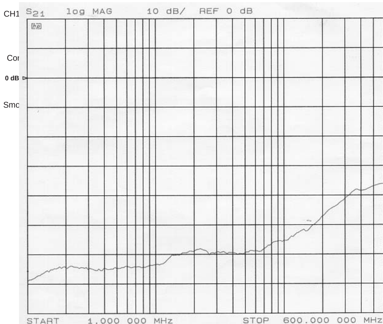
Figure 26. Crosstalk of the CB3Q3306A at 3-pF Load ( V_{CC} = 3.3 V)
