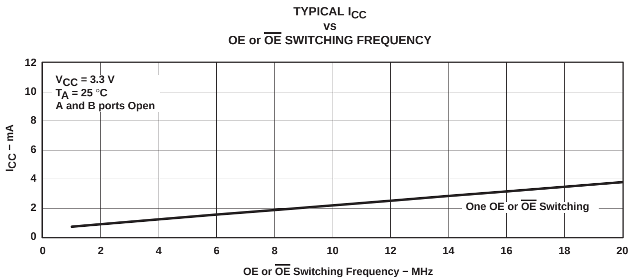
Figure 2. Typical I_{CC} vs OE or \overline{OE} Switching Frequency, V_{CC} = 3.3\text{ V}
