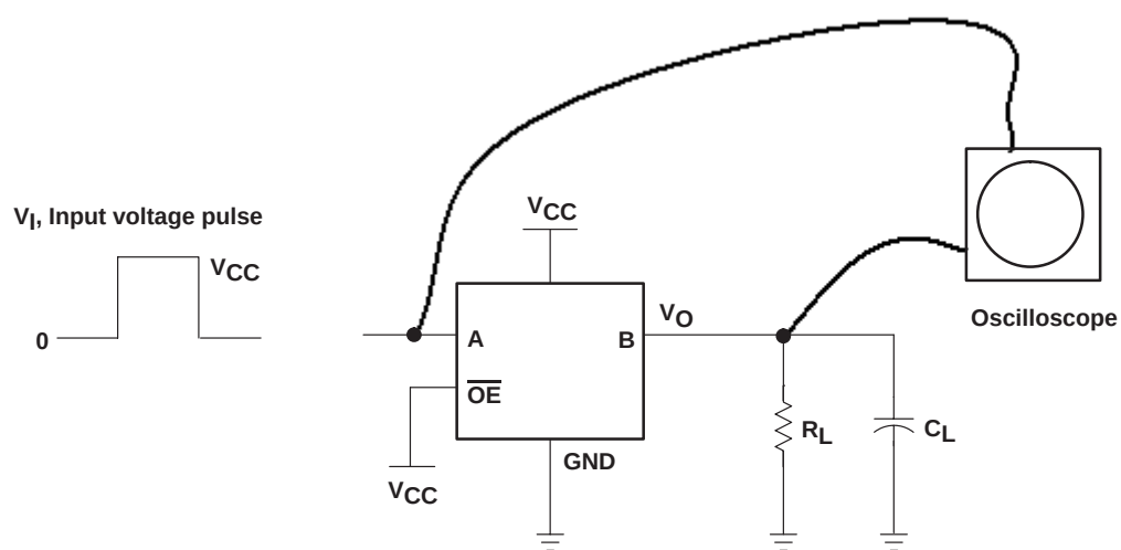
Figure A-4. Voltage-Time Waveform Measurement (Switch Off)
