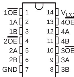
DGX OR PW PACKAGE (TOP VIEW)
