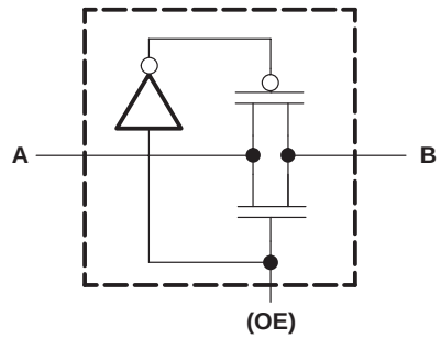
Simplified Schematic of Each FET Switch (SW)
