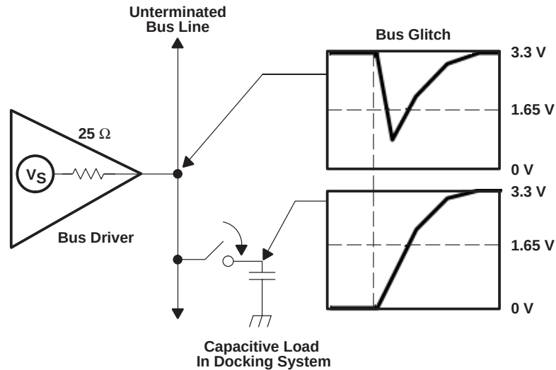
Figure 2. Bus Glitch
