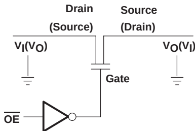
Figure 3. NMOS Series Switch
