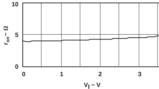
Figure 8. r_{on} vs V_I in an NMOS Series Switch With the Charge Pump ( V_{CC} = 3.6 V)
