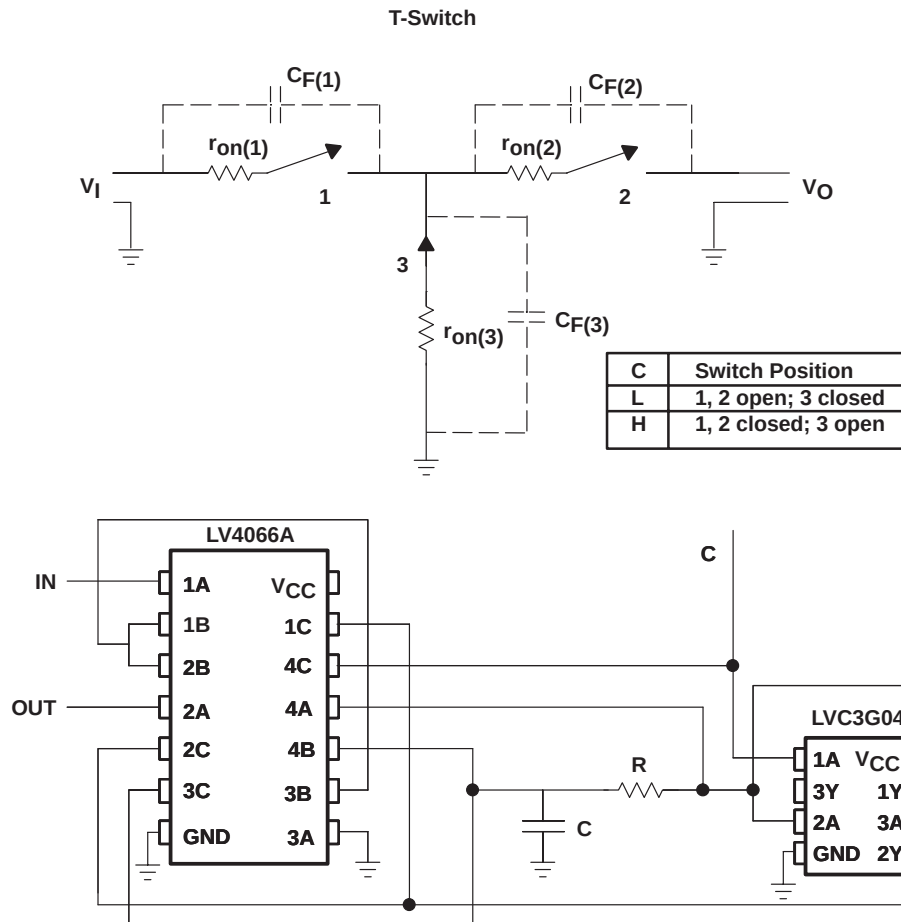
Figure 51. LV4066A/LVC2G04 T-Switch Configuration
