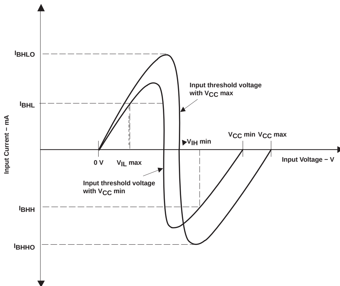
Figure 26. Bus-Hold Currents
