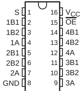
DBQ, DGV, OR PW PACKAGE (TOP VIEW)
