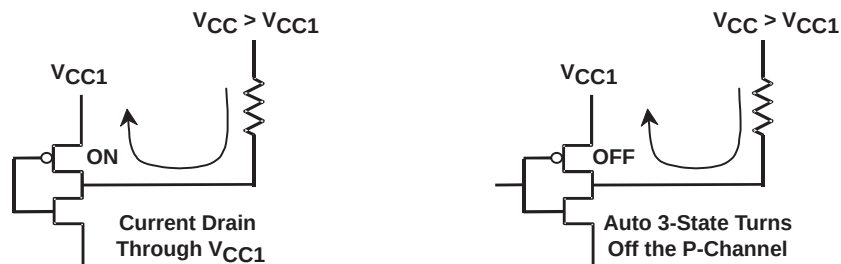
Figure 15. Auto3-State
