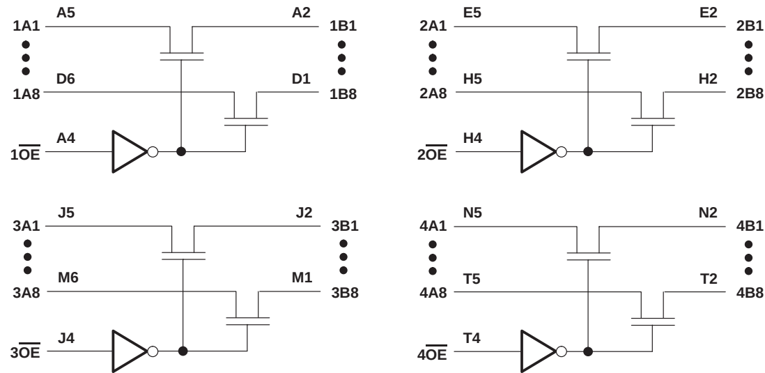
logic diagram (positive logic)
