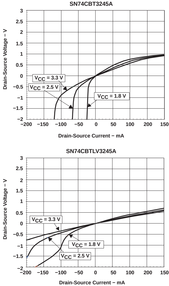
Figure 10. Low-State r_{on} of CBT3245A and CBTLV3245A at Different Supply Voltages
