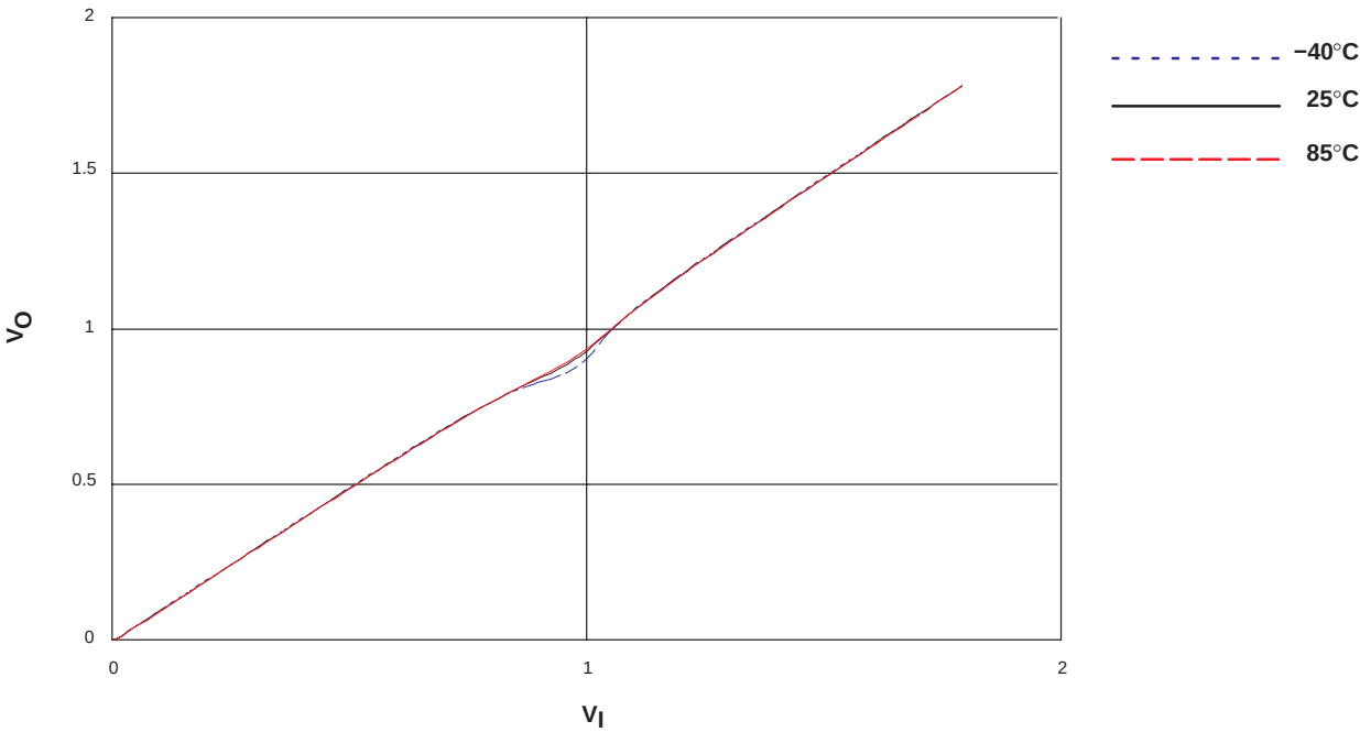
Figure 38. V_O vs V_I , V_{CC} = 1.8 V (SN74LVC1G66)
