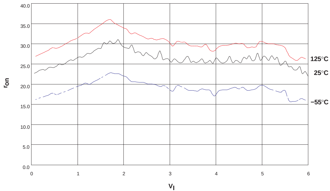
Figure 15. r_{on} vs V_I , V_{CC} = 6\text{ V} (CD74HC4066)
