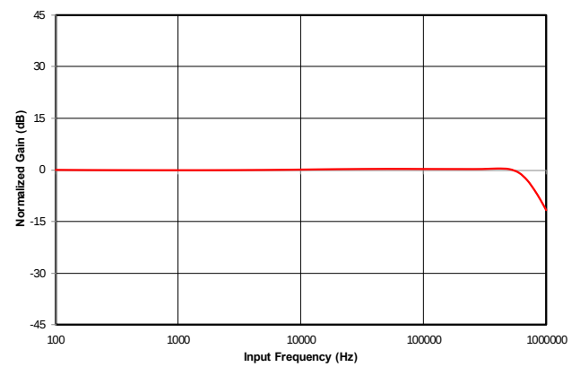
Figure 4.25. Amplifier Bandwidth
