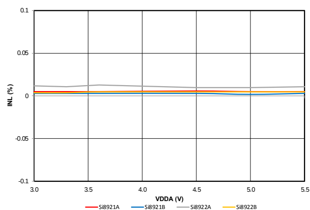
Figure 4.5. Nonlinearity (%) vs. VDDA Supply (V)
