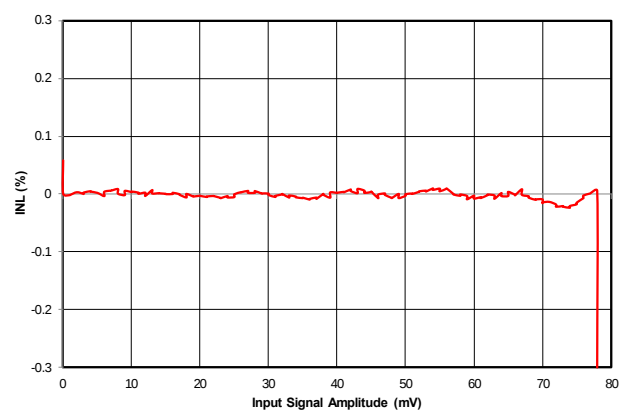
Figure 4.9. Si8922A Nonlinearity (%) vs. Input Signal Amplitude (mV)
