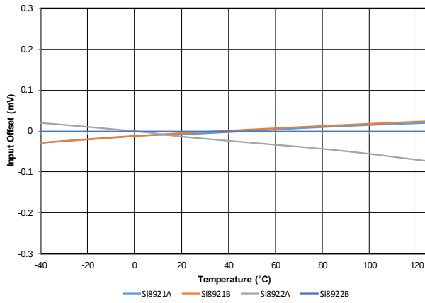
Figure 4.22. Input Offset (mV) vs. Temperature (°C)
