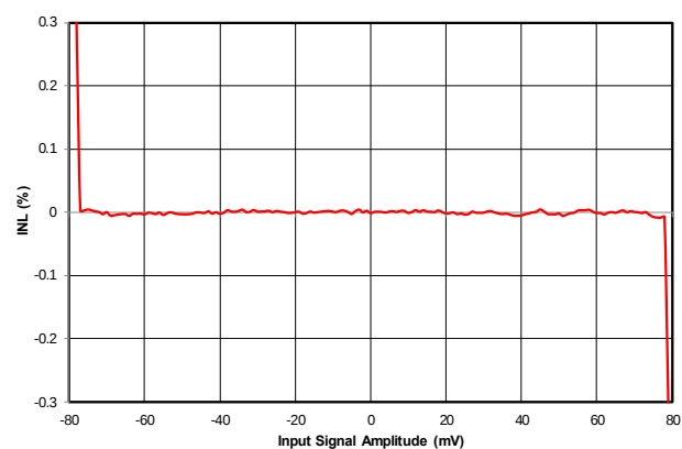
Figure 4.7. Si8921A Nonlinearity (%) vs. Input Signal Amplitude (mV)
