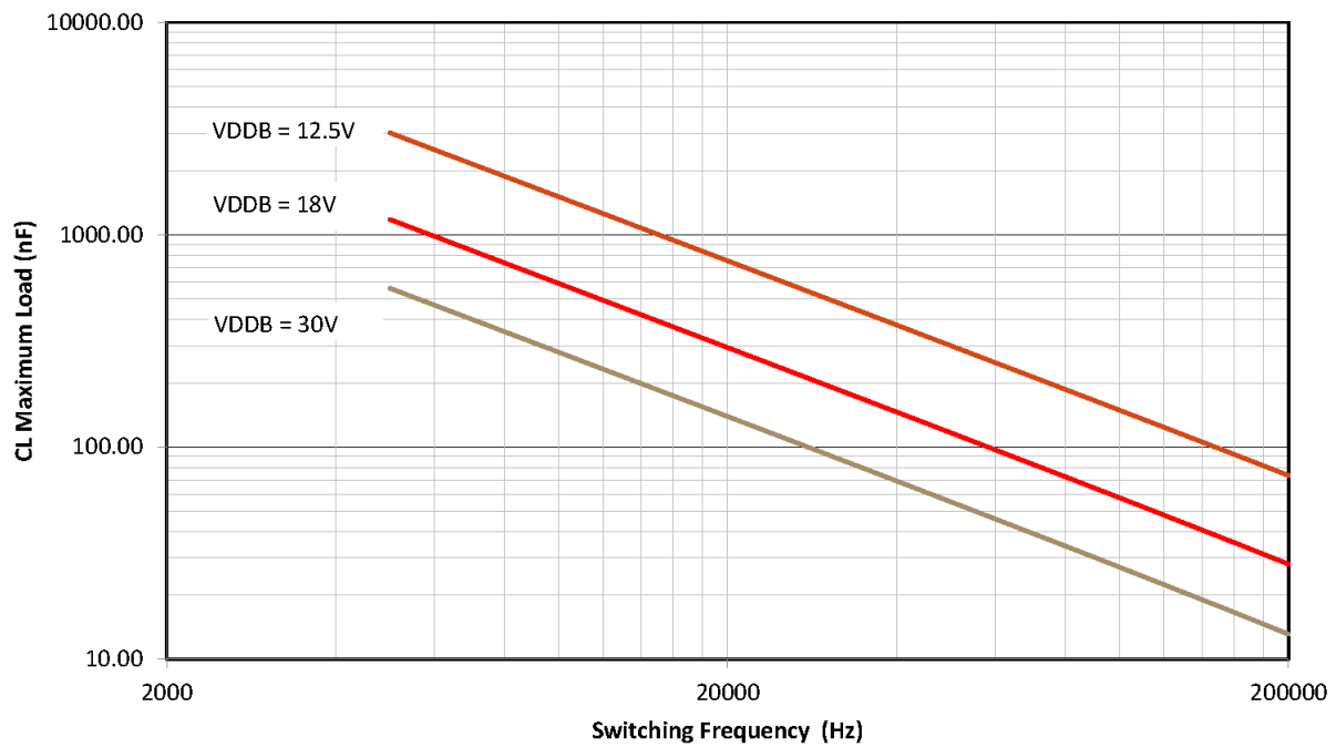
Figure 3.3. Maximum Load vs. Switching Frequency (25 °C)
