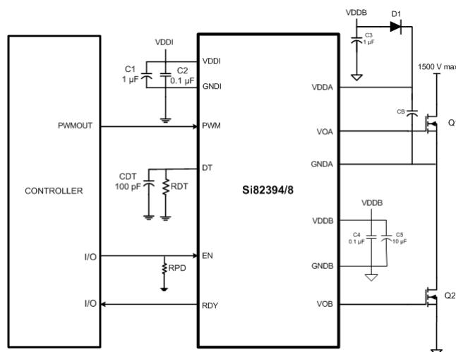
Figure 3.1. Si82394/8 in Half-Bridge Application
