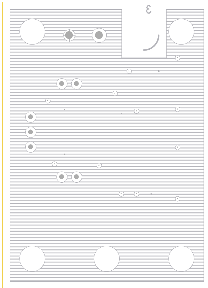
Figure 7. Layer 4: PWR
