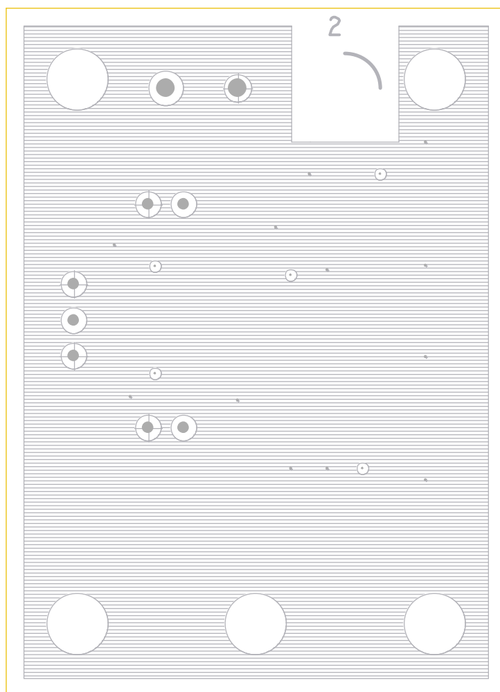
Figure 6. Layer 2: GND
