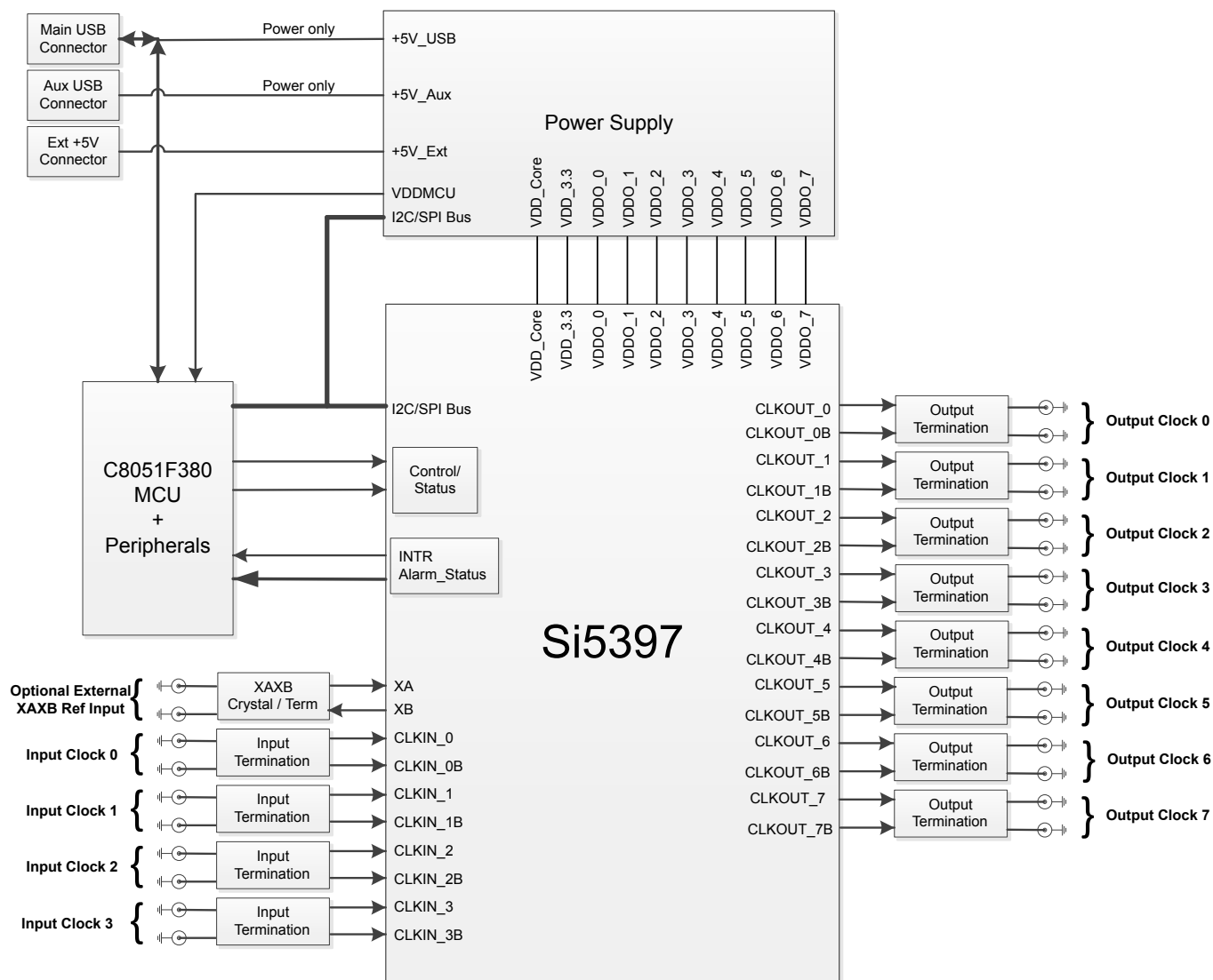
Figure 1.1. Si5397 EVB Functional Block Diagram
