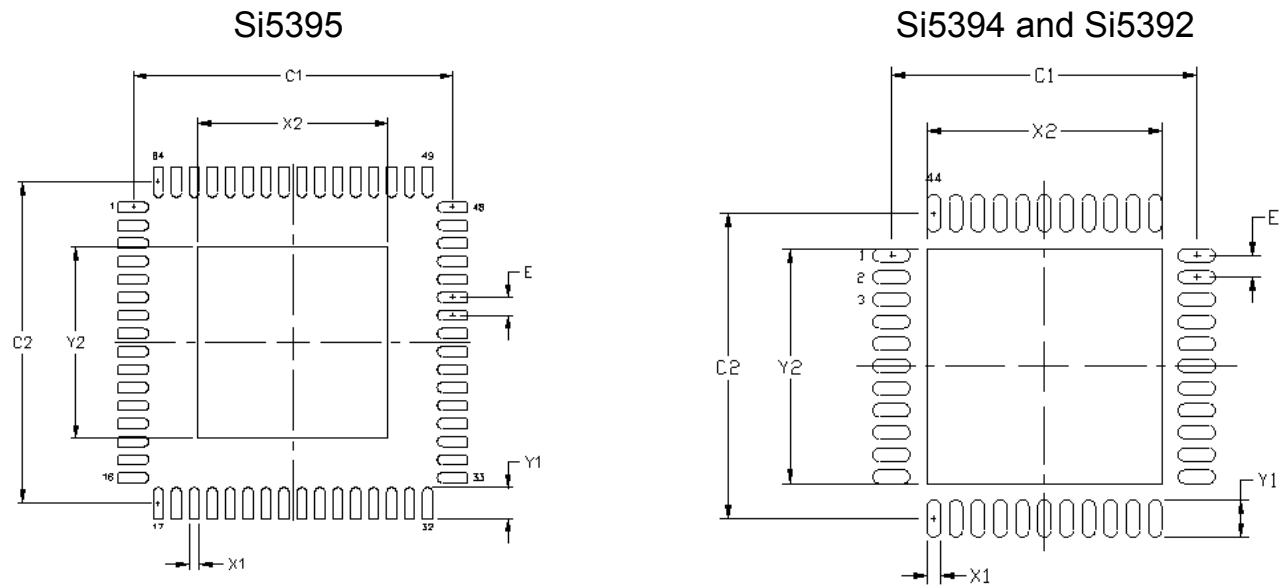
Figure 11.1. PCB Land Pattern
