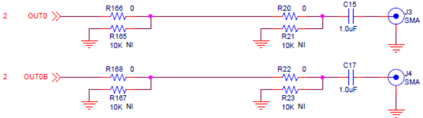
Figure 8.1. Output Clock Termination Circuit
