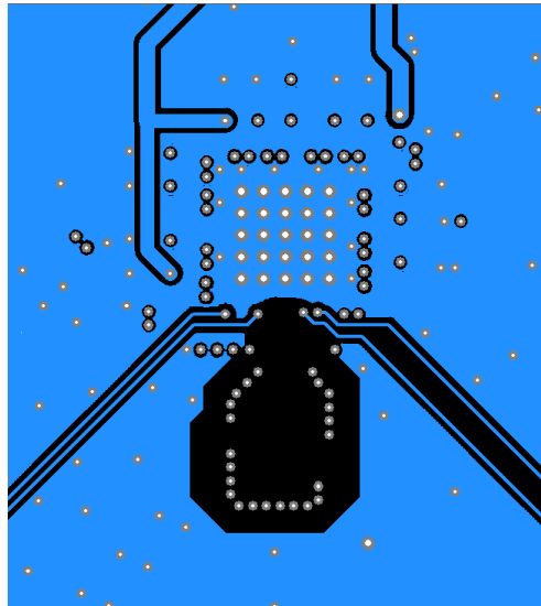
Figure 10.4. Power Plane (Layer 4)
