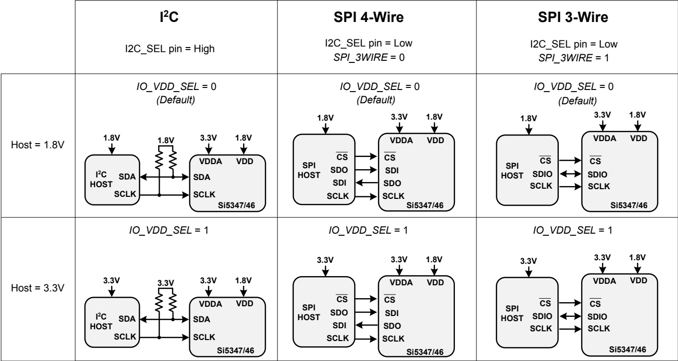
Figure 7.1. I 2 C/SPI Device Connectivity Configurations
