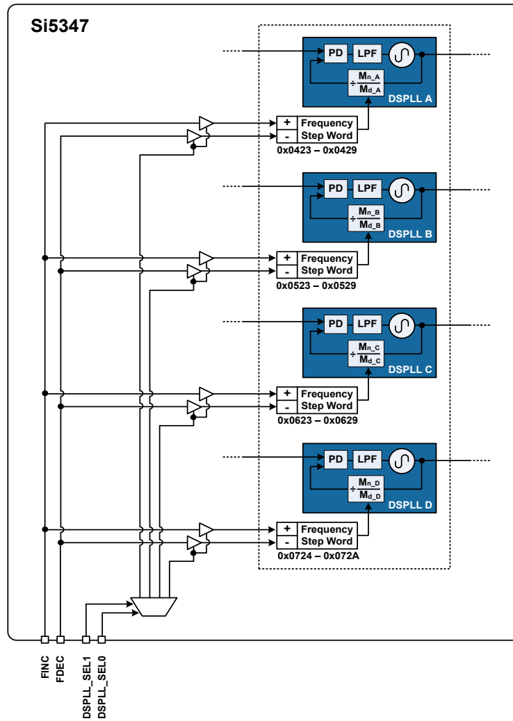
Figure 6.1. Controlling the DCO Mode By Pin Control
