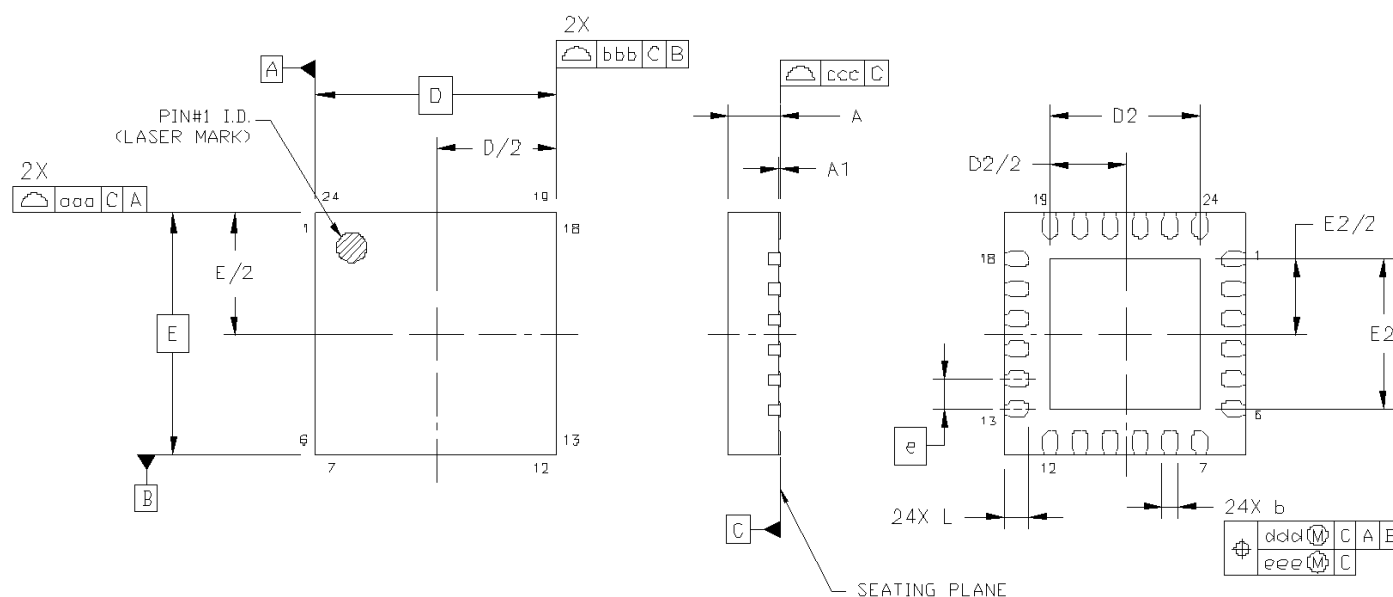
Figure 6.2. 24-Pin QFN Package
