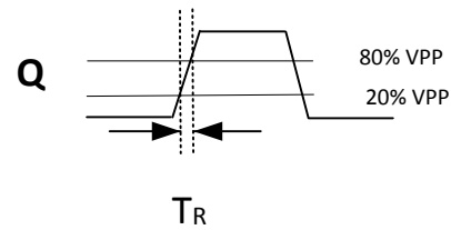
Rise/Fall Time
