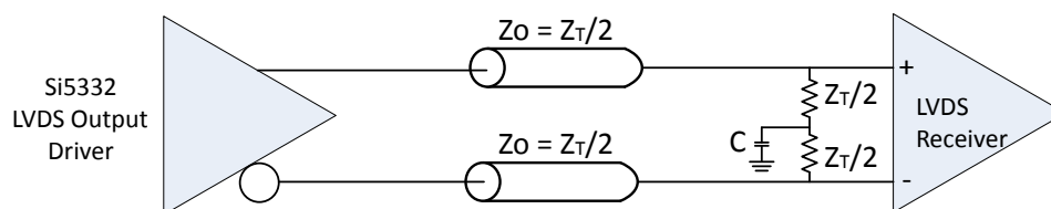
Figure 3.5. Optional LVDS Termination
