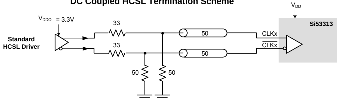
Figure 5. Differential DC-Coupled Input Terminations
