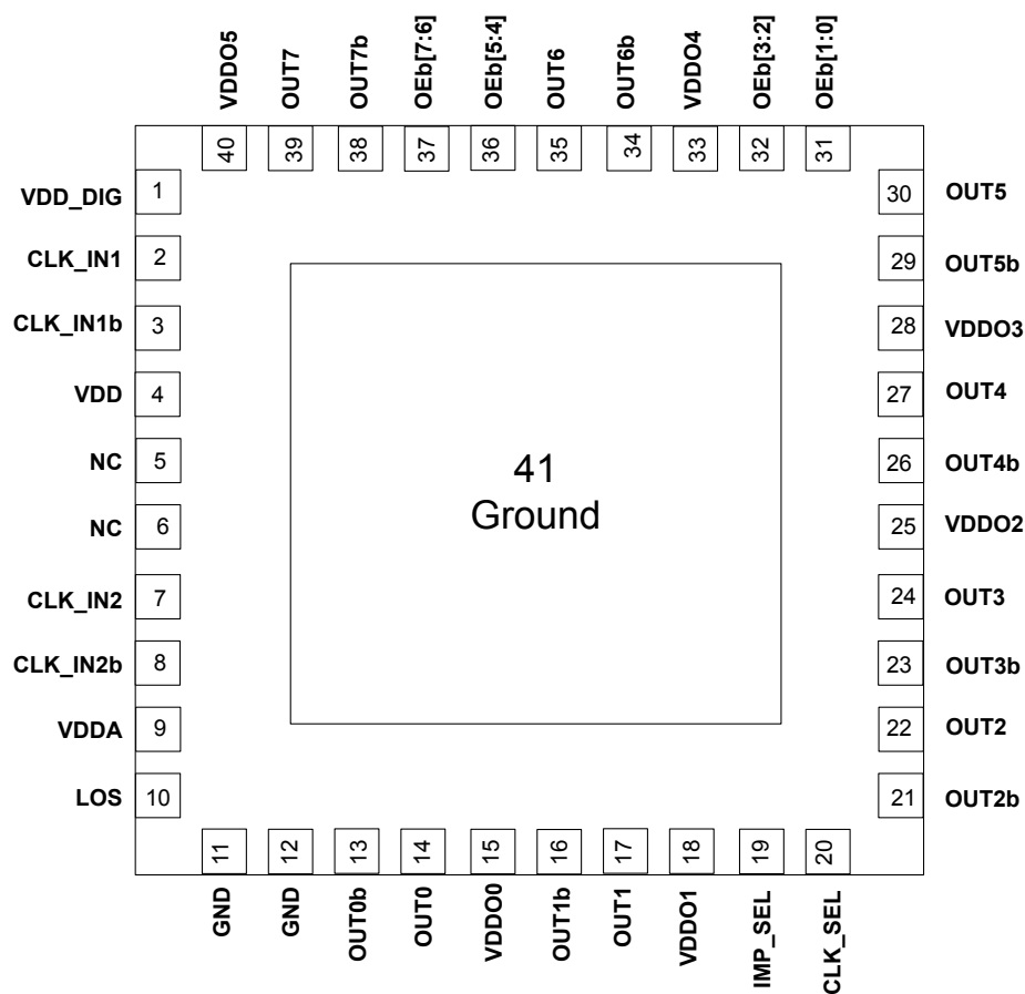
Figure 6.2. Si53258A-D02-AM 40-QFN
