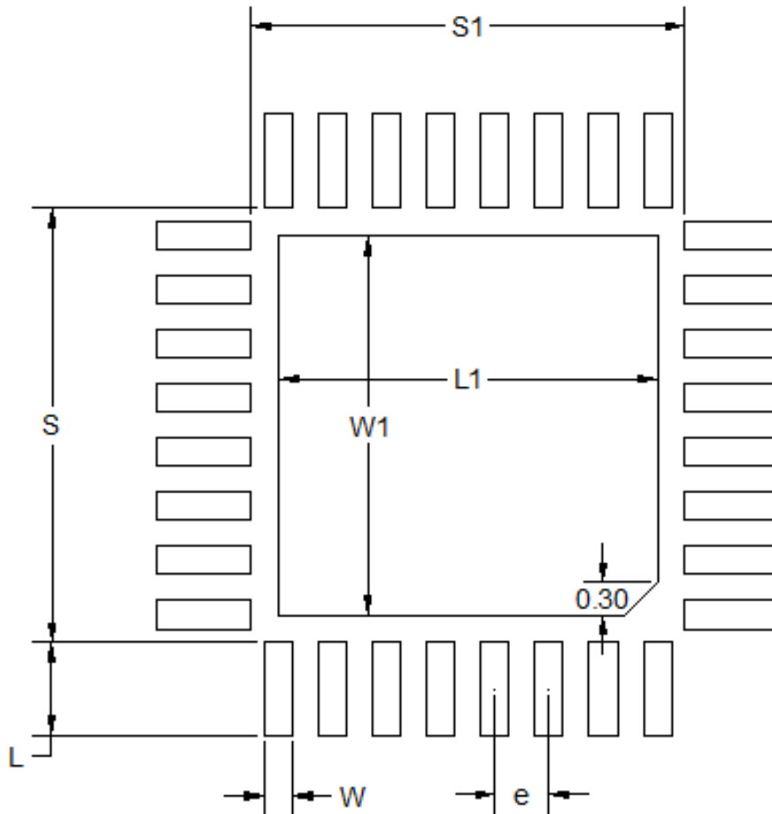
Figure 6. Land Pattern
