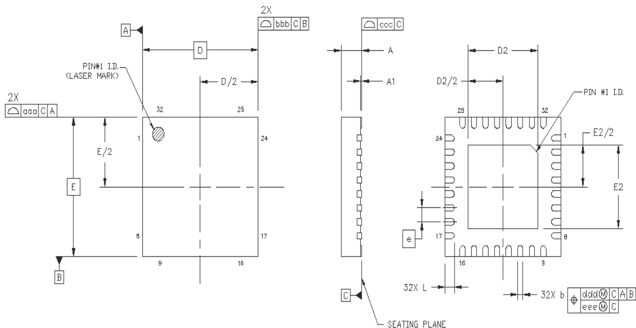
Figure 5. 32-Pin Quad Flat No Lead (QFN) Package
