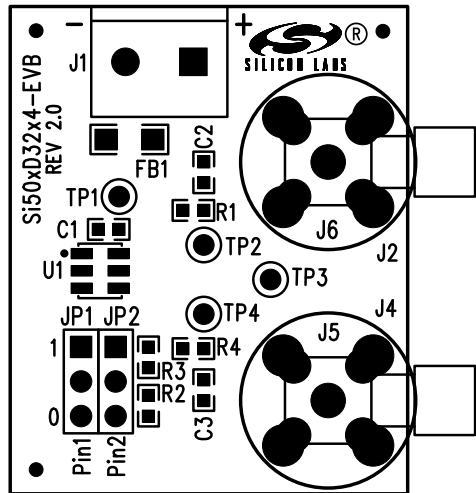
Figure 4. Assembly Drawing
