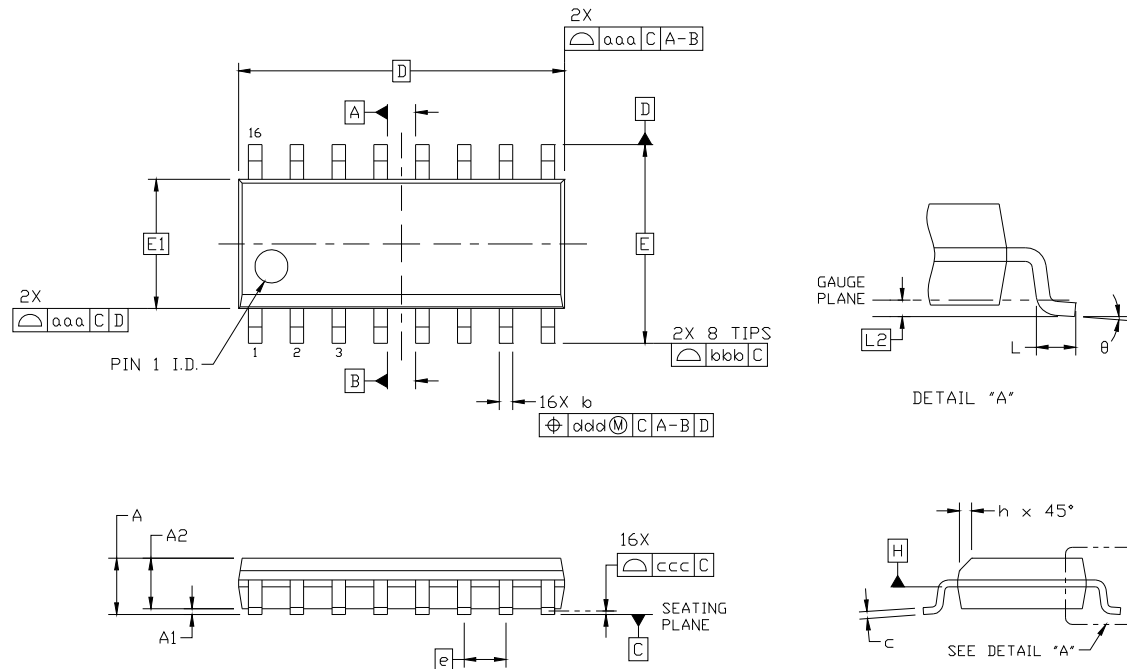
Figure 3. 16-Pin SOIC
