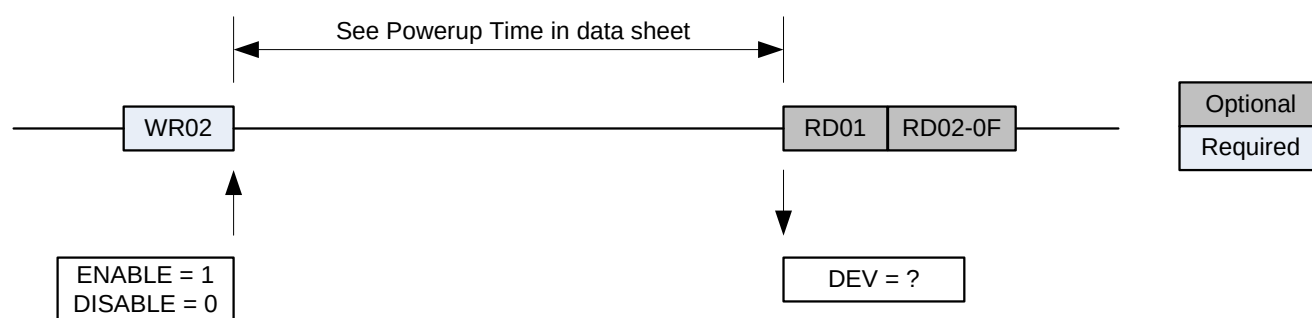
Figure 4. Powerup Timing
