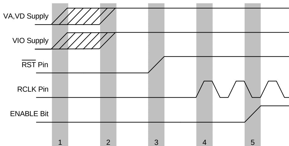
Figure 1. Initialization Sequence
