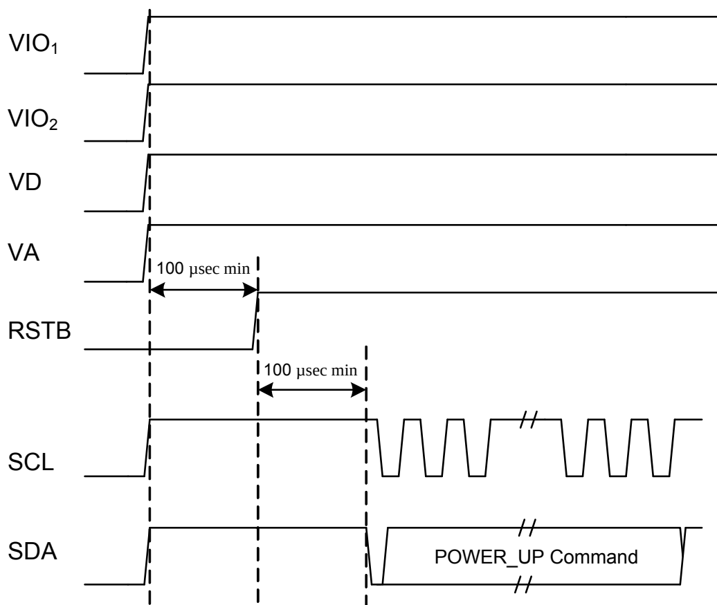
Figure 27. Startup Timing
