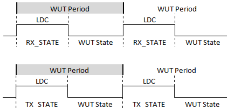
Figure 11. RX LDC Sequences
