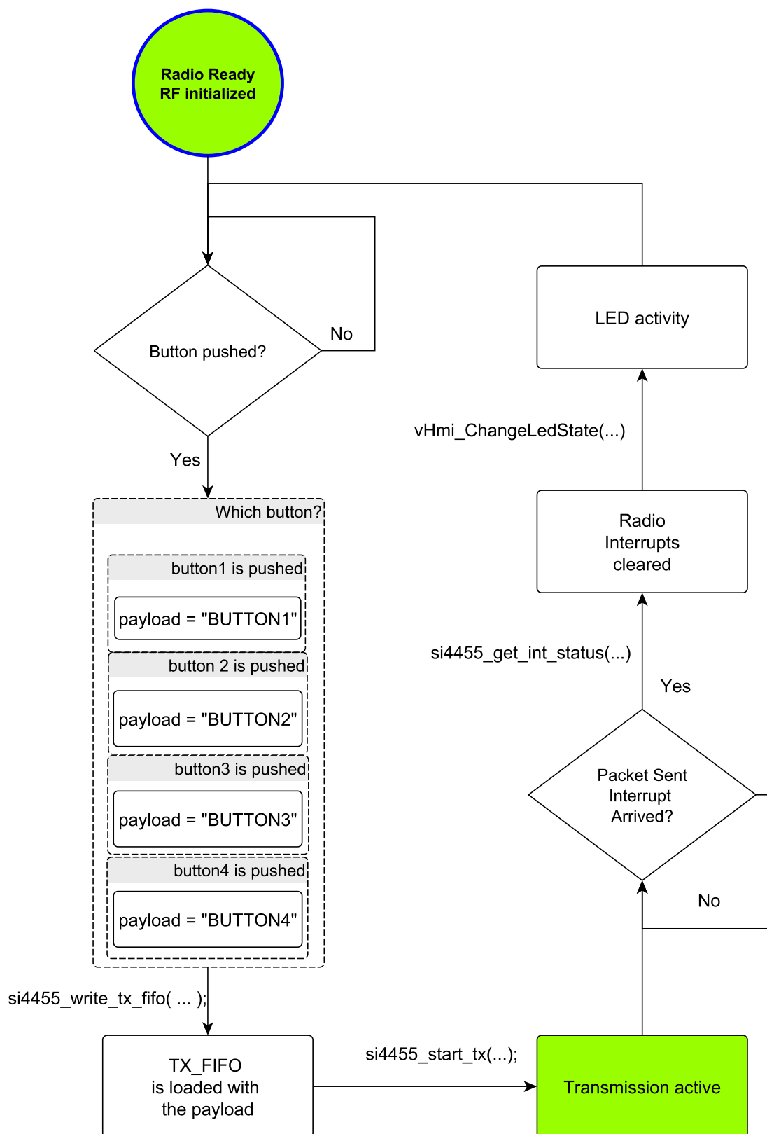
Figure 32. Transmission Flowchart
