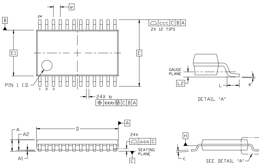
Figure 21. 24-Pin Thin Shrink Small Outline Package (TSSOP)
