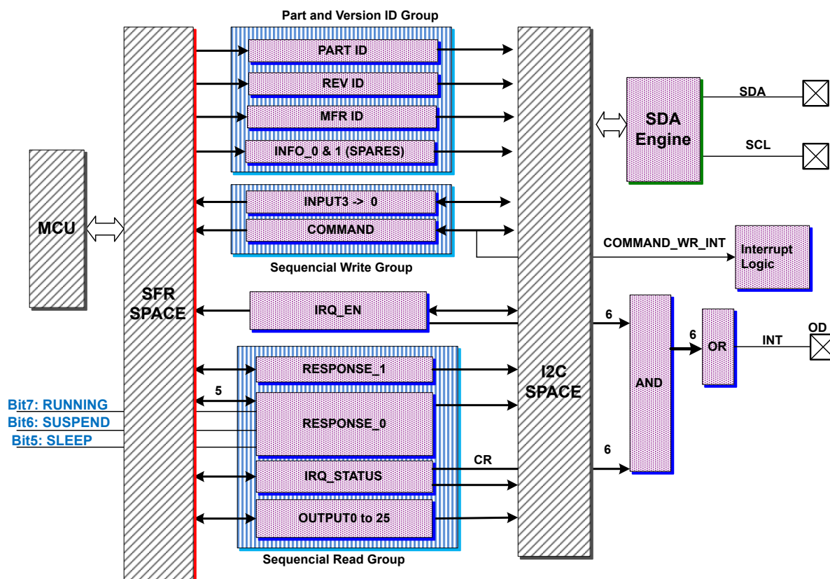
Figure 5.1. I 2 C Interface Block Diagram
