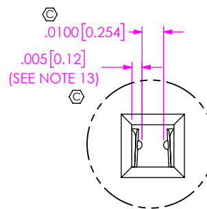
DETAIL 'D' SCALE 16:1
