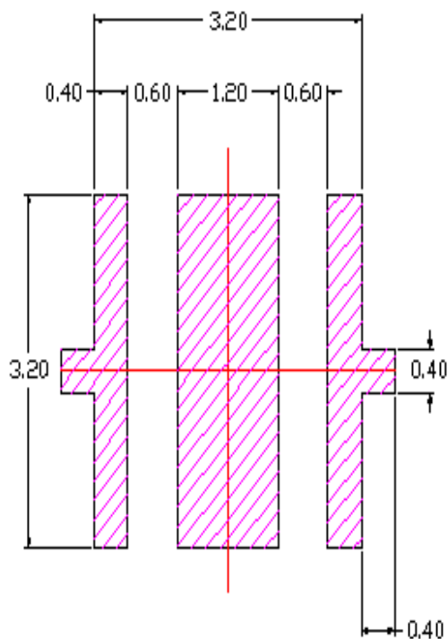
Recommended Stencil Pattern
