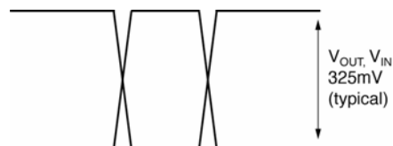
Figure 2c. Single-Ended Swing
