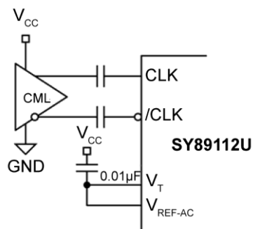
Figure 11. CML Interface (AC-Coupled)
