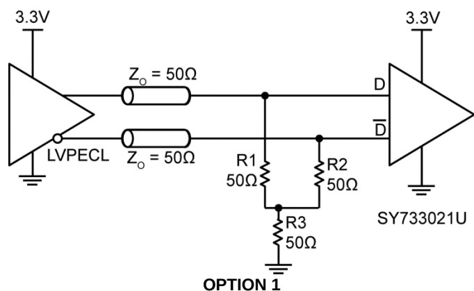
D, /D Input Driven by a 3.3V LVPECL Driver
