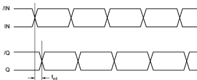
Figure 1. Propagation Delay
