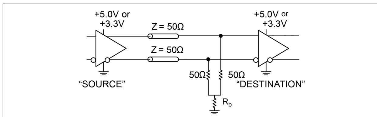
FIGURE 4-2: Three-Resistor Y-Termination.
