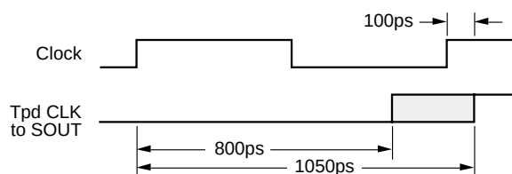
Figure 2. Cascaded 1:8 Converter Architecture
