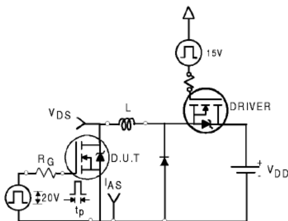
Fig. 16. Unclamped Inductive switching test circuit & waveform
