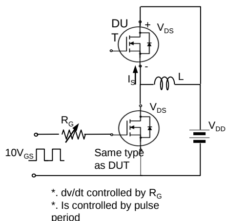
Fig. 17. Peak diode recovery dv/dt test circuit & waveform
