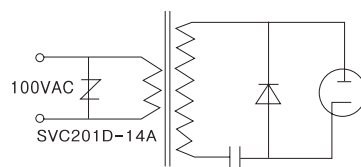
Triac protection
