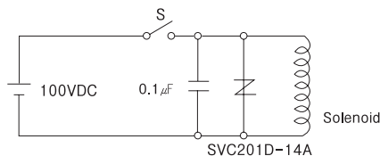
Contact protection
