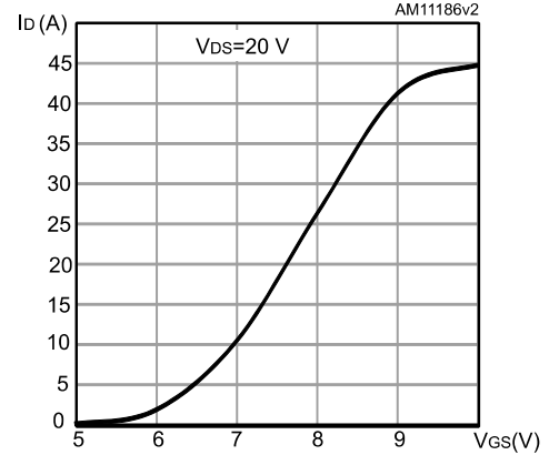
Figure 9: Transfer characteristics
