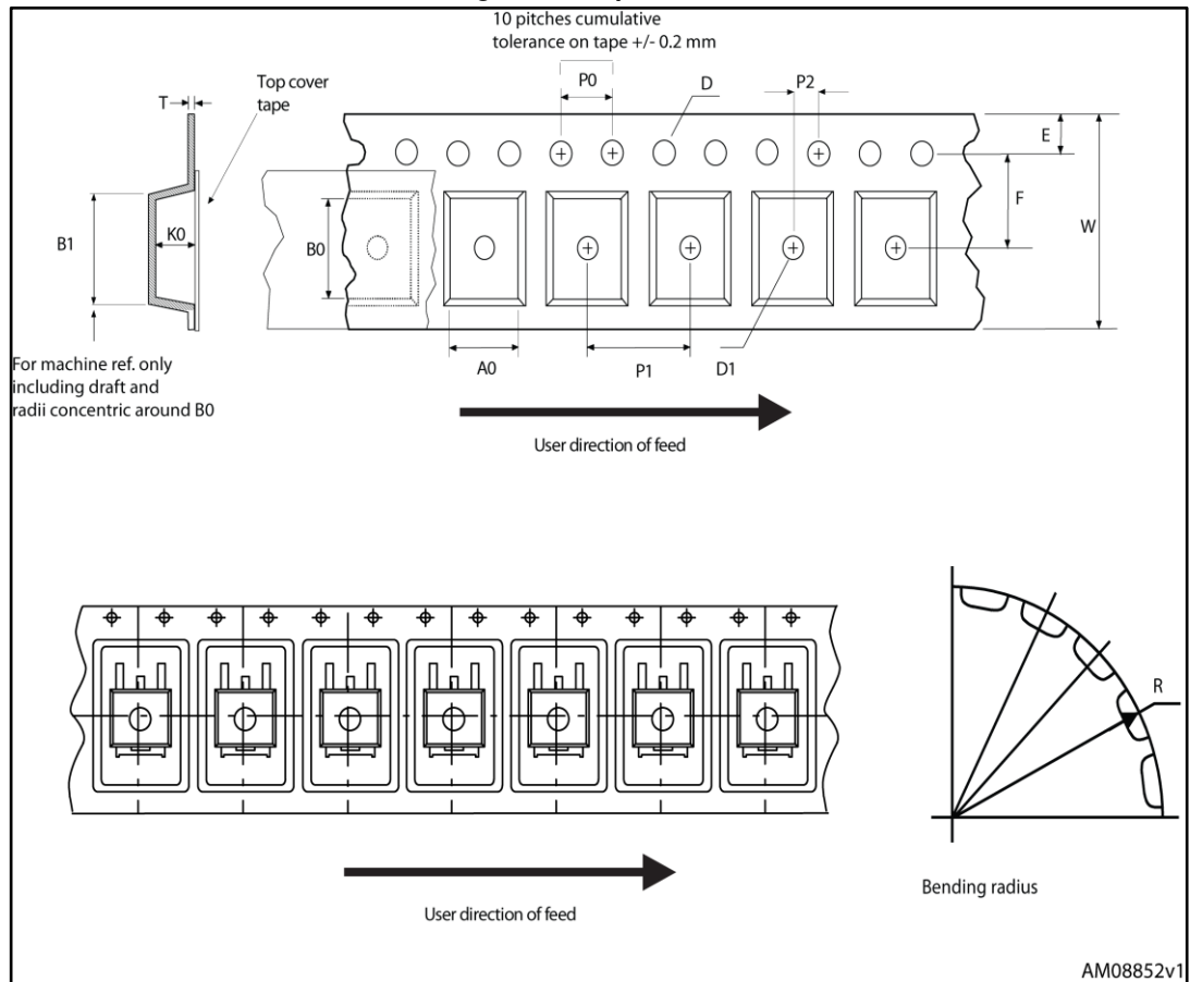
Figure 30: Tape outline
