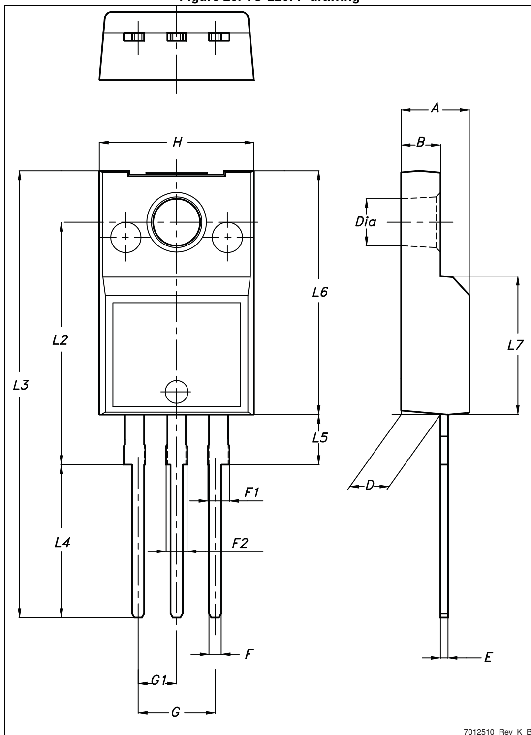
Figure 26. TO-220FP drawing
