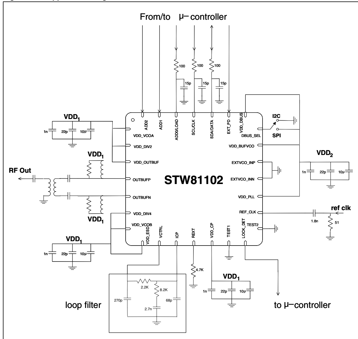
Figure 36. Application diagram
