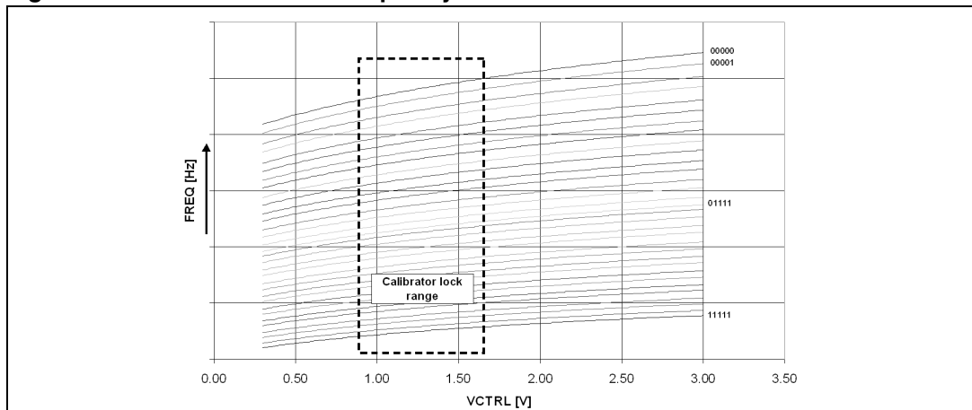
Figure 19. VCO Sub-Bands Frequency Characteristics
