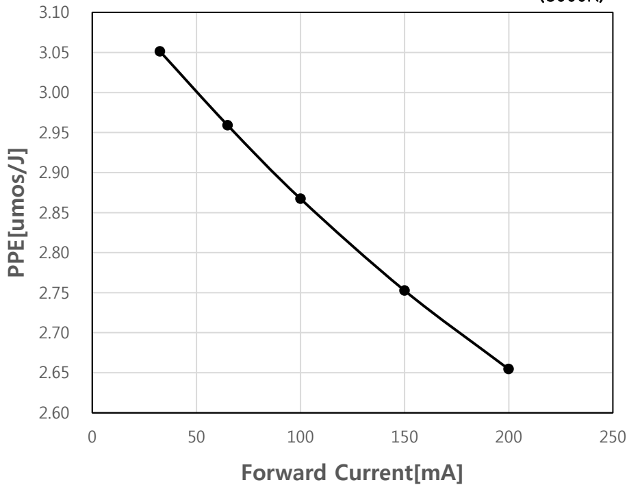
Fig 11. Forward Current vs. Photosynthetic Photon Energy , T_j = 25^{\circ}\text{C} (3000K)
