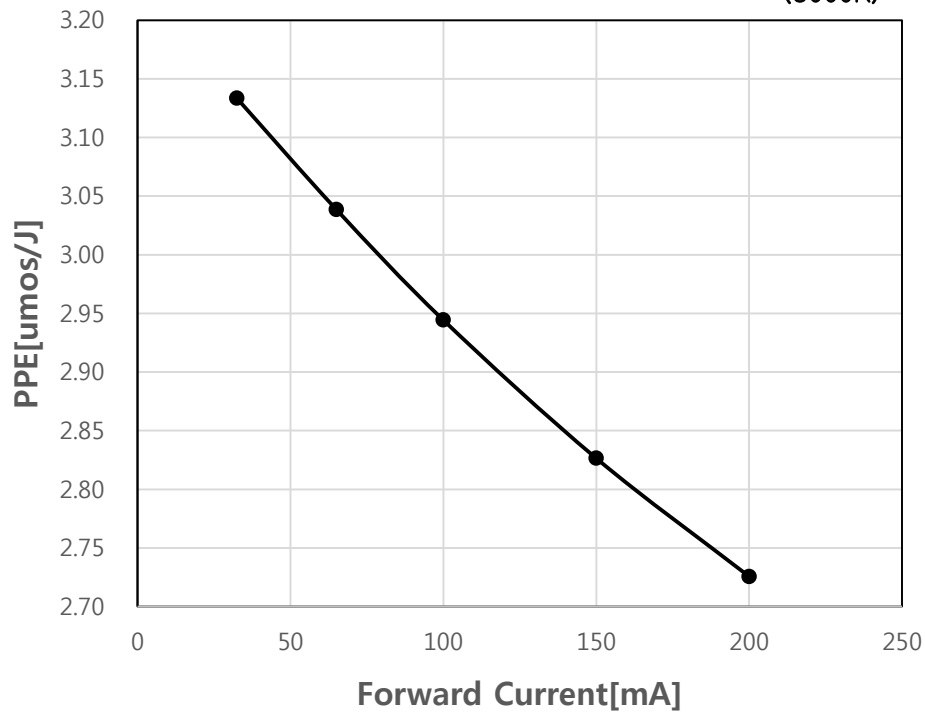
Fig 11. Forward Current vs. Photosynthetic Photon Energy , T_j = 25^{\circ}\text{C} (5000K)
