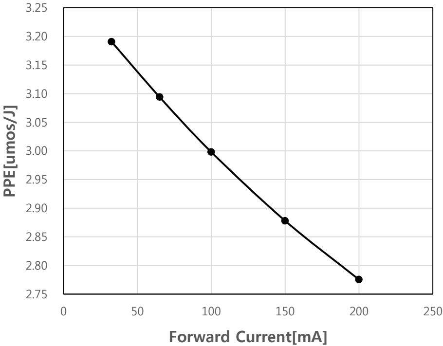
Fig 11. Forward Current vs. Photosynthetic Photon Energy , T_j = 25^{\circ}\text{C} (6500K)
