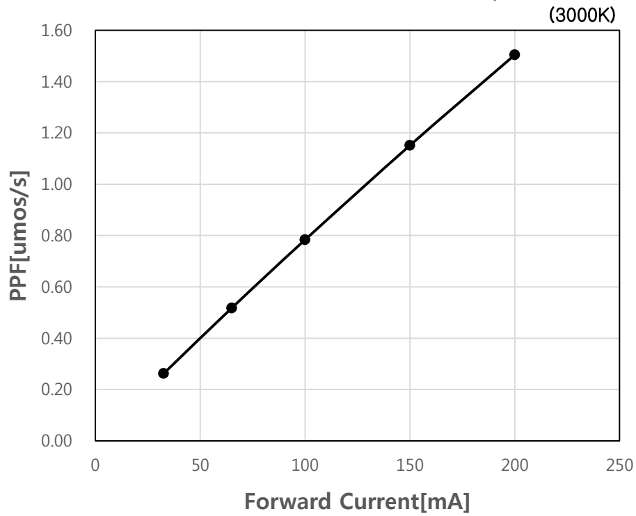
Fig 10. Forward Current vs. Photosynthetic Photon Flux, T_j = 25^\circ\text{C}
