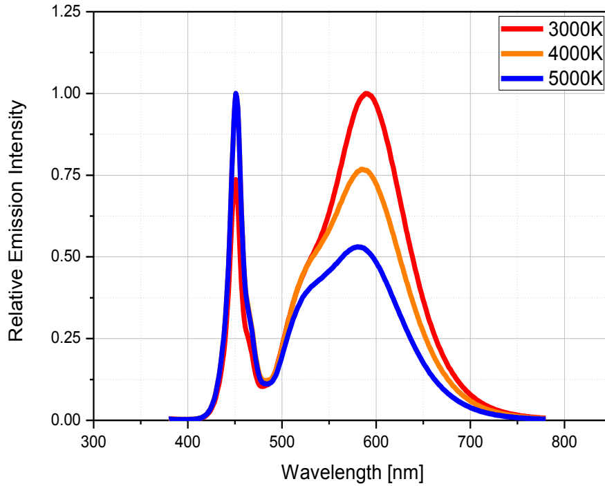
Fig 1. Color Spectrum, T_j = 25^\circ\text{C}
