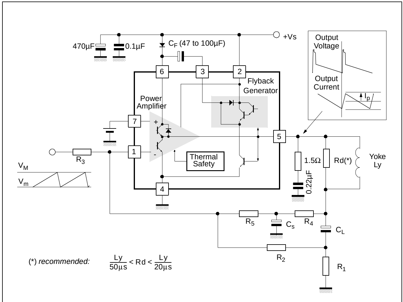
Figure 6: AC-coupled Application
