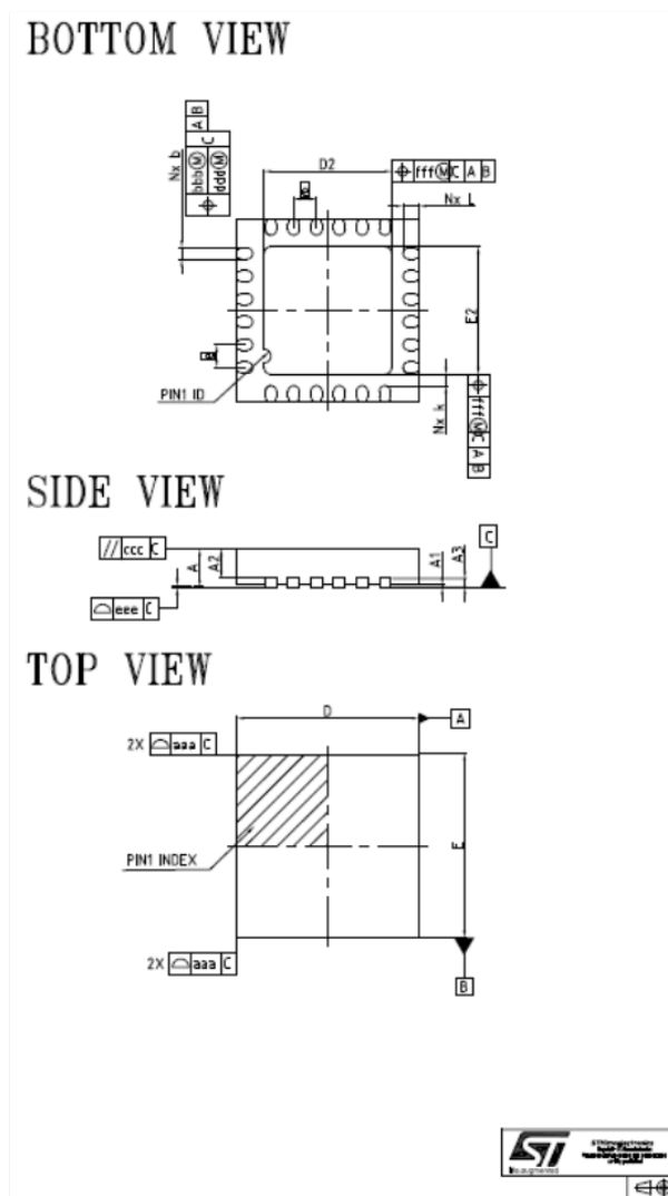
Figure 10. QFN24 EP 4x4 mm package outline
