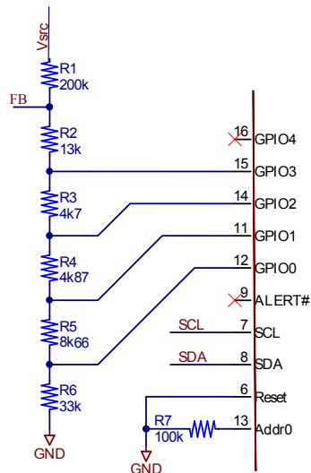
Figure 7. Power supply - buck topology extract
