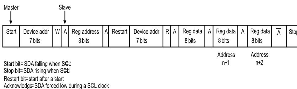
Figure 3. Read operation
