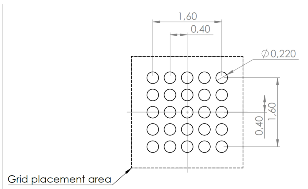
Figure 12. WLCSP (2.6x2.6x0.5) recommended footprint
