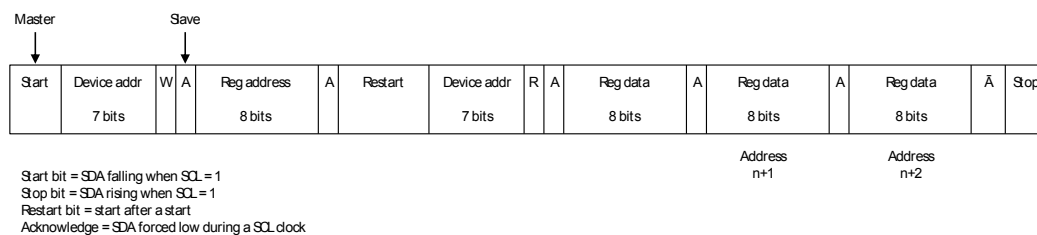
Figure 4. Read operation
