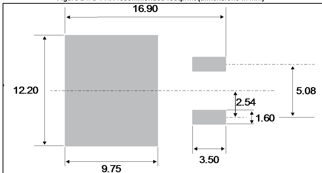
Figure 14: D 2 PAK recommended footprint (dimensions in mm)
