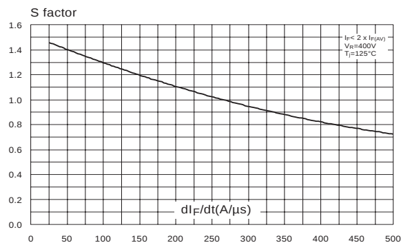
Figure 7: Reverse recovery softness factor versus dl_F/dt (typical values, per diode)
