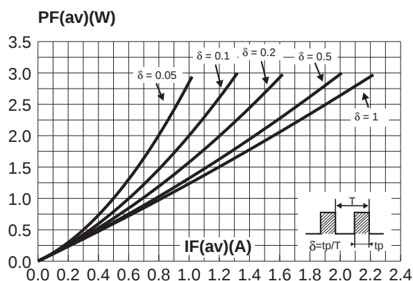
Fig. 1: Power dissipation versus average forward current.
