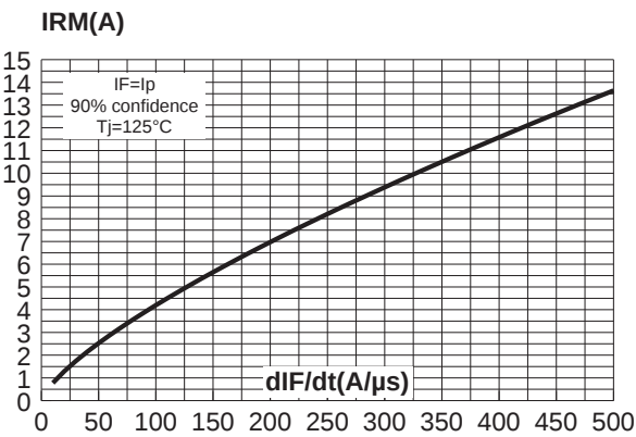
Fig. 6: Reverse recovery current versus dI_F/dt .
