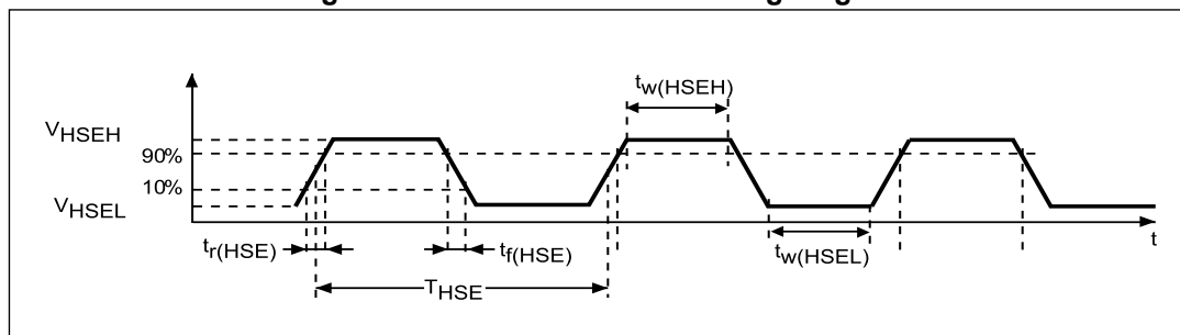
Figure 11. HSE clock source timing diagram
