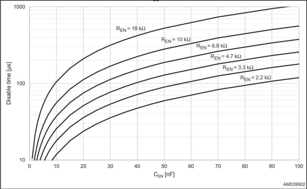
Figure 9. Disable time versus R_{EN} and C_{EN} values ( V_{DD} = 3.3\text{ V} )
