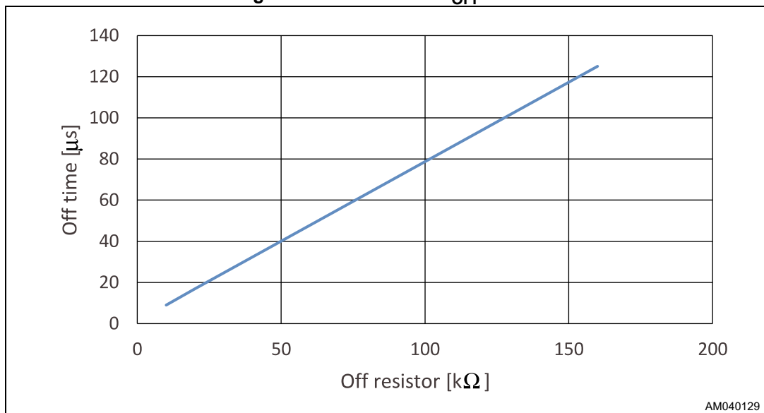
Figure 7. OFF time vs. R_{\text{OFF}} value
