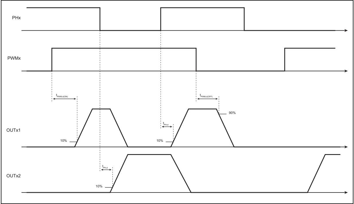
Figure 4. Timing diagram
