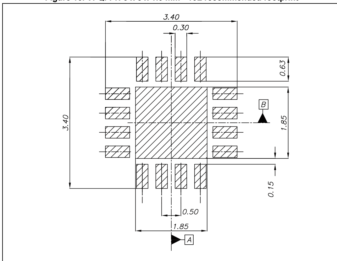
Figure 16. VFQFPN 3 x 3 x 1.0 mm - 16L recommended footprint
