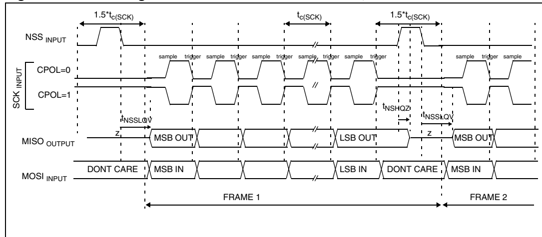
Figure 35. SPI configuration, slave mode with CPHA=1, single transfer
