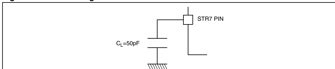
Figure 6. Pin loading conditions
