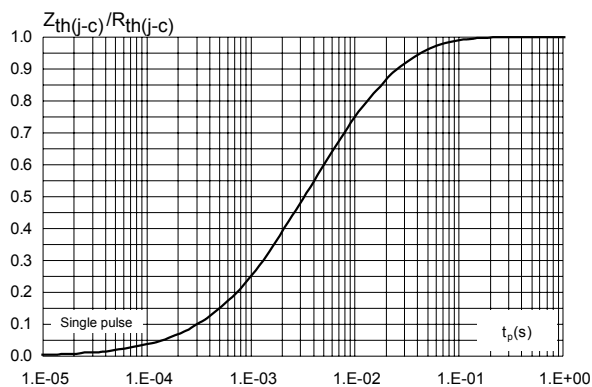
Figure 7. Relative variation of thermal impedance junction to case versus pulse duration (TO-220AC, DPAK and D 2 PAK)
