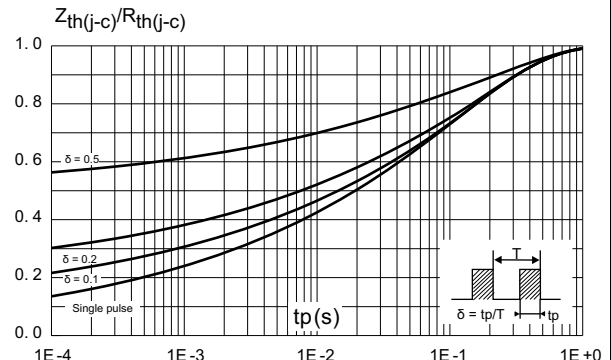
Figure 6. Relative variation of thermal transient impedance junction to case versus pulse duration
