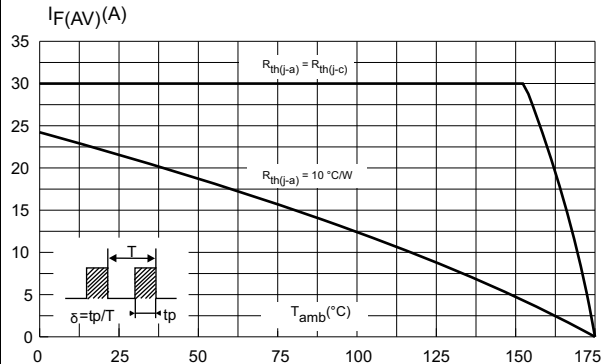
Figure 2. Average current versus ambient temperature ( \delta = 0.5 , per diode)
