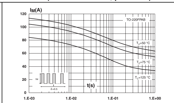
Figure 6. Non repetitive surge peak forward current versus overload duration (maximum values, per diode)
